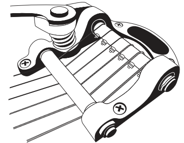
Figure 15: Bigsby Vibrato
