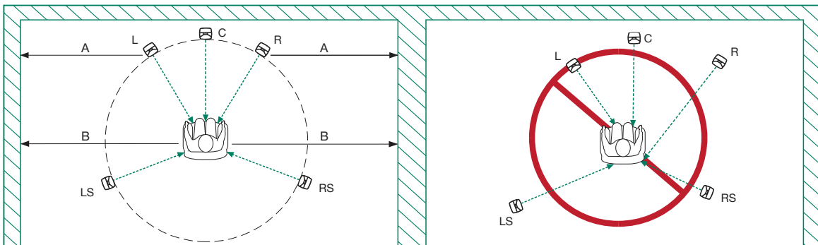
Symmetry of Room Installation
