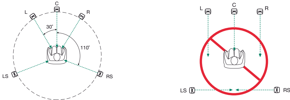
Speaker Angle and Distance
