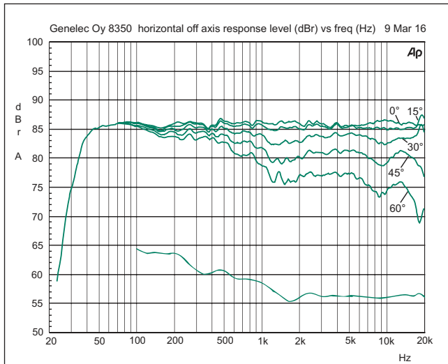
Figure 14. The upper curve group shows the horizontal directivity characteristics of the 8350A measured at 1 m. The lower curve shows the system’s power response.
