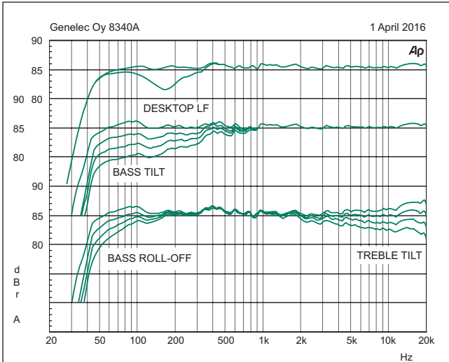
Figure 11. The curves above show the effect of the “Bass Tilt”, “Treble Tilt”, “Desktop Low Frequency” and “Bass Roll-Off” controls on the free field response of the 8340A.
