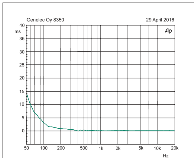
Figure 15. The curve above shows the delay variation of the 8350A as a function of frequency.
