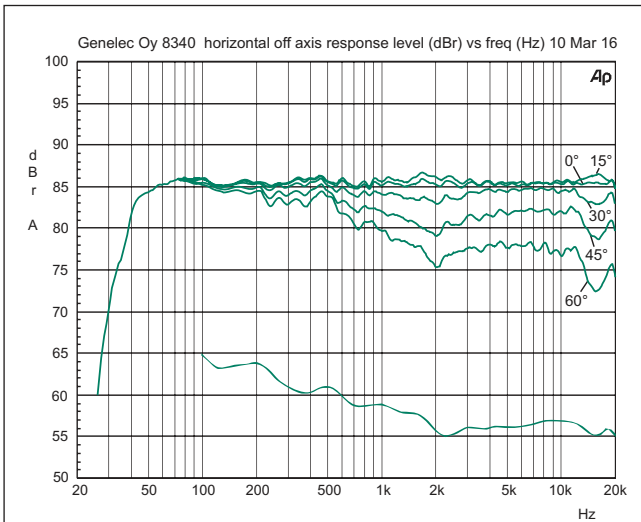
Figure 13. The upper curve group shows the horizontal directivity characteristics of the 8340A measured at 1 m. The lower curve shows the system’s power response.
