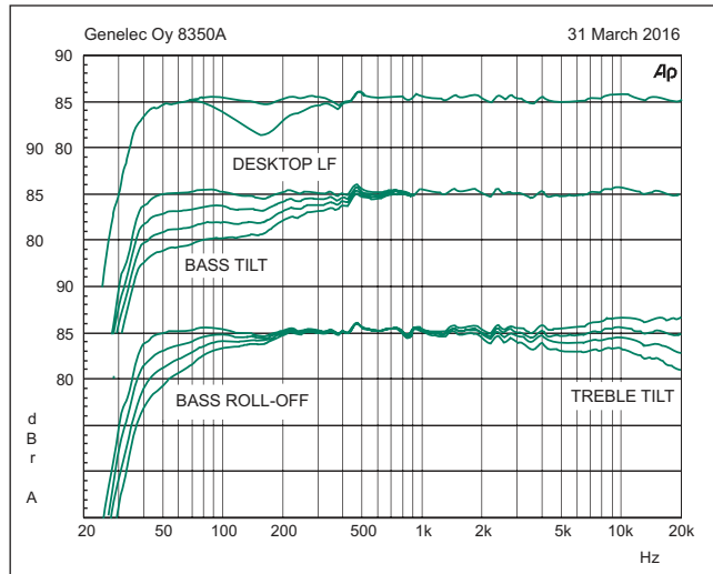
Figure 12. The curves above show the effect of the “Bass Tilt”, “Treble Tilt”, “Desktop Low Frequency” and “Bass Roll-Off” controls on the free field response of the 8350A.
