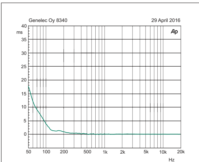
Figure 14. The curve above shows the delay variation of the 8340A as a function of frequency.
